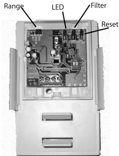
Figure 1 PIR with cover removed
