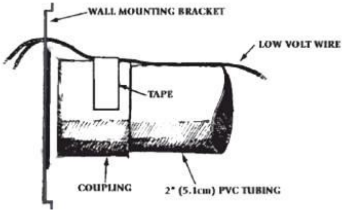
Fig. 02 Inner-Wall Closet Assembly
